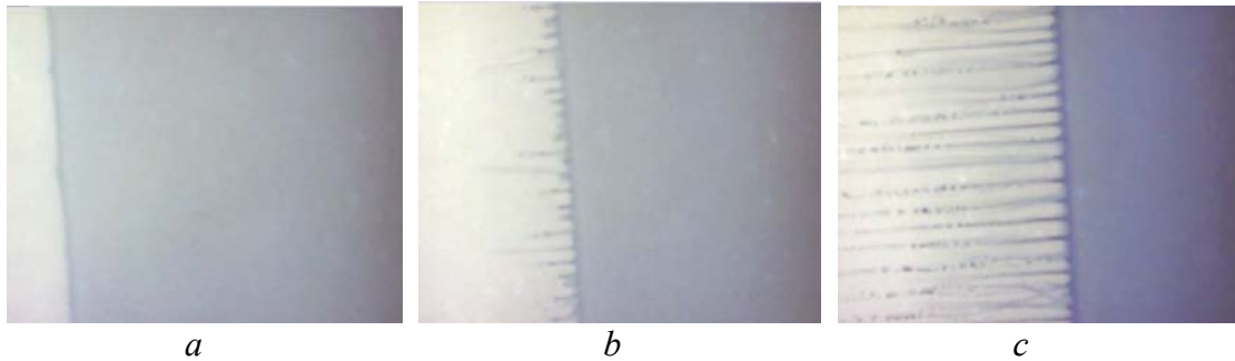
Fig. 2: Formation of periodic structure during solidification of an aqueous solution bromtimol blue. a - flat interphase boundary, b - emergence of concentration distortion, c - formed periodic structure.
