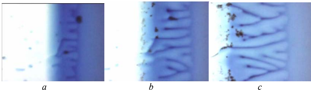
Fig. 3: The formation of periodic structures in a thin layer of an aqueous solution bromtimol blue. A - beginning of structure formation, b, c - process of structure formation.
