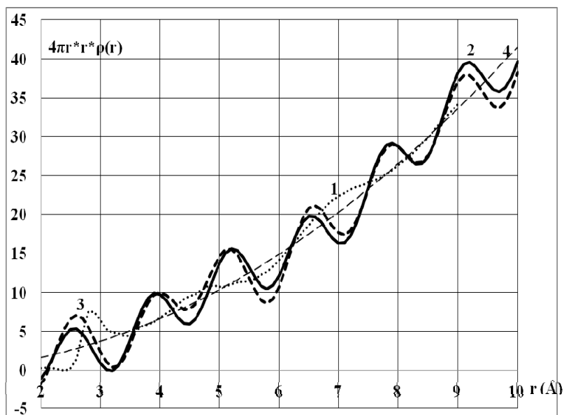
Figure1: Functions of radial distribution: 1) water [2]; 2) amorphous ice -3^{\circ}\text{C} ; 3) amorphous ice -160^{\circ}\text{C} ; 4) 4\pi r^3 \rho_0(r) - average value of electron density fluctuations.
